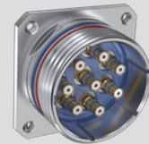
233-290-HS Wall Mount Receptacle, Standard Helicoils (Pin Contacts)
