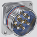
233-290-CS Wall Mount Receptacle, Standard Clinch Nuts (Pin Contacts)
