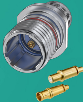
Series 806 RF Micro miniature multi-port circular
