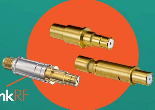
G-Link RF : 26.5 GHz RF BMB-to-SMA contact adapters
