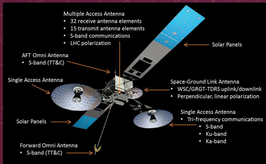
Third-Generation Tracking and Data Relay Satellite (TRDS) Capabilities. Note the numerous antenna types and functions. (Source: NASA)
