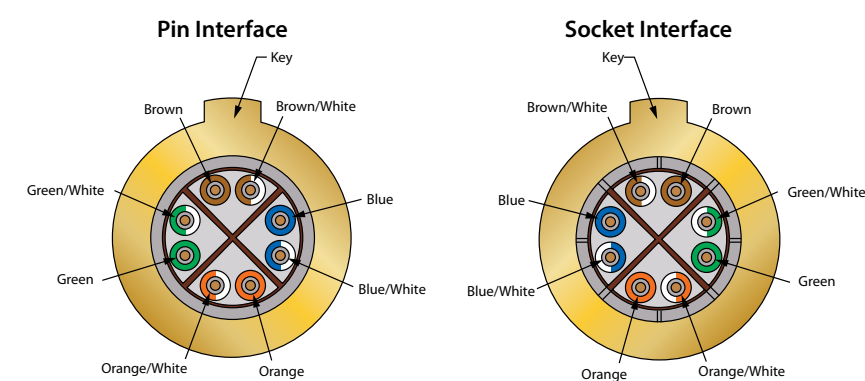
Recommended wire-to-contact assignments
