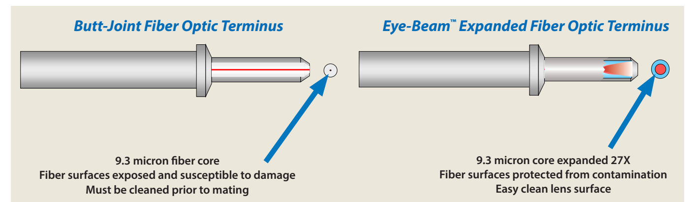
Eye-Beam termini and factory-terminated jumpers may be integrated into a broad range of circular and rectangular connector packaging
