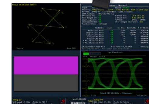
SMPTE 3G - SDI at +90°C Pathological Case 3
