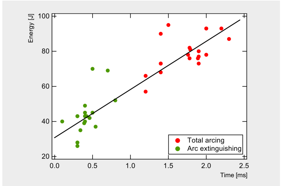
Figure 5: The correlation between arcing time and arc energy is shown over all measured pressure groups. The red and green points represent data for the total arcing and the arc extinguishing processes, respectively. A linear fit is shown as solid line and the linear correlation parameter is r = 0.9 .
