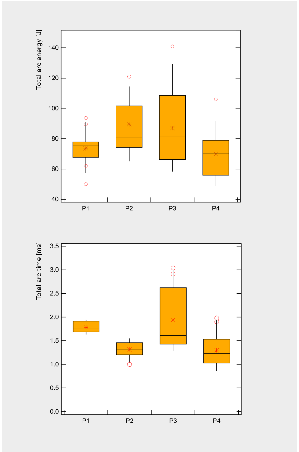
Figure 7: Boxplots showing total arc energy and arc time for different gas pressures P1-P4 within the arcing chamber. Red circles indicate outliers and asterisks the average values.
