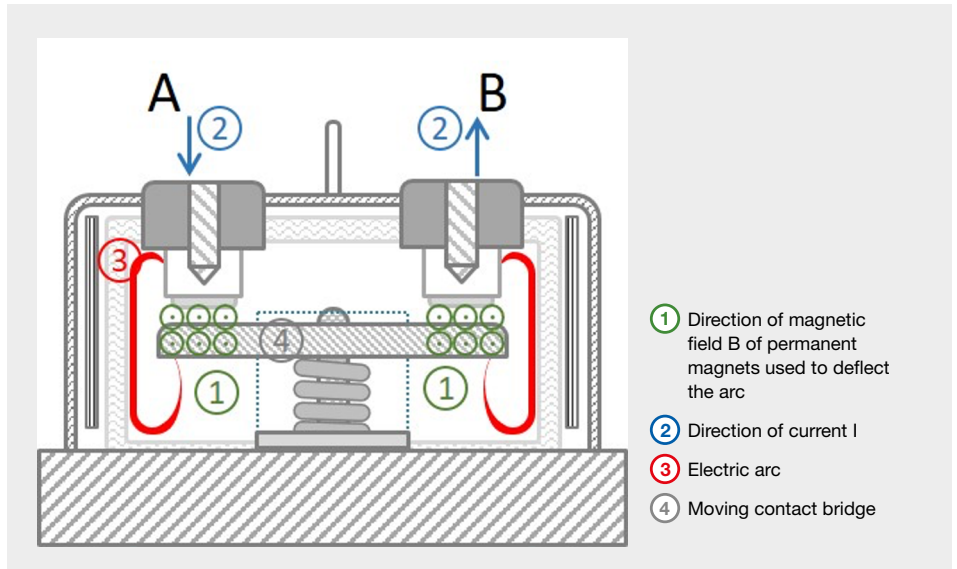
Figure 2: General principle of gas-filled contactor – inside view
