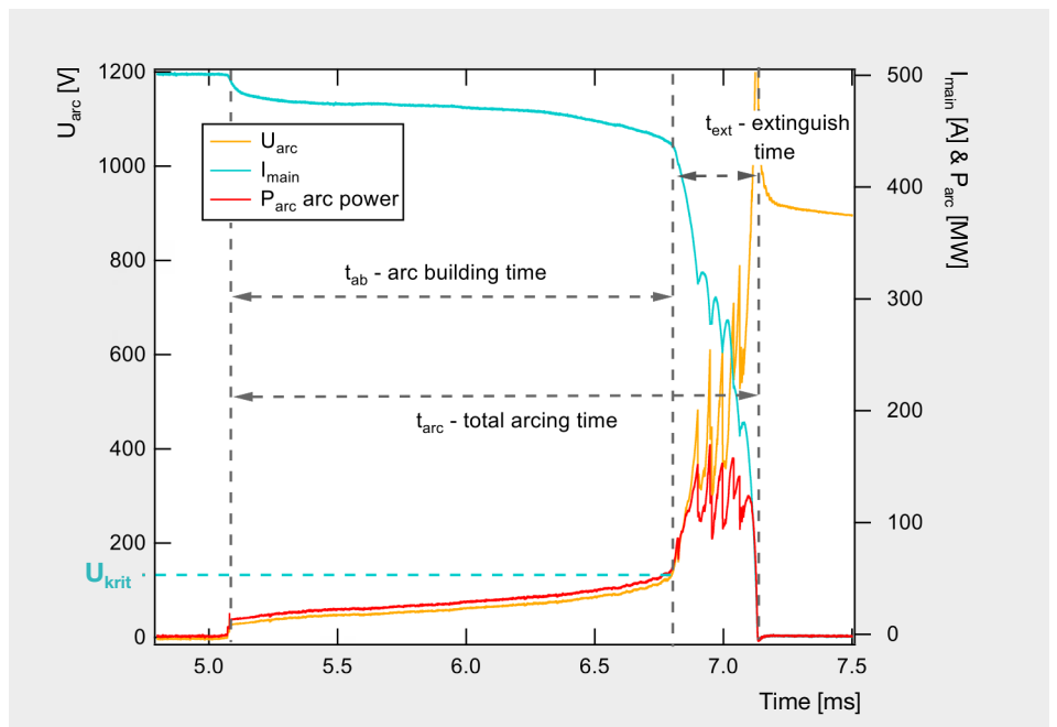
Figure 4: A magnified view of the arcing process in Figure 3 is shown. The total arcing time is divided into two characteristic time intervals: t_{ab} when arc voltage is built up and t_{ext} as the time, in which the arc is extinguished.
