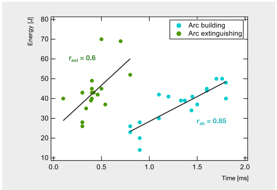
Figure 6: Correlation analysis between arc energy and time of arc building (blue) and extinguishing (green) processes. The extinguishing process is faster but still consumes about the same energy as the arc building process, which is generally longer.
