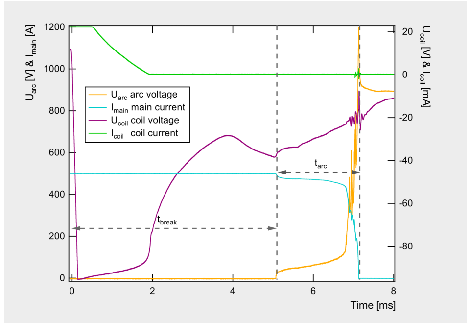
Figure 3: The break process is shown exemplarily with U_{arc} and I_{main} as the voltage and current at the main contacts (left axis) and U_{coil} and I_{coil} as accordingly for the coil (right axis). I_{coil} is shifted by a factor of 10 for better clarity. The time between switching off the coil and the mechanical opening of the main contacts is defined as t_{break} and the actual arcing time is then given by t_{arc} .
