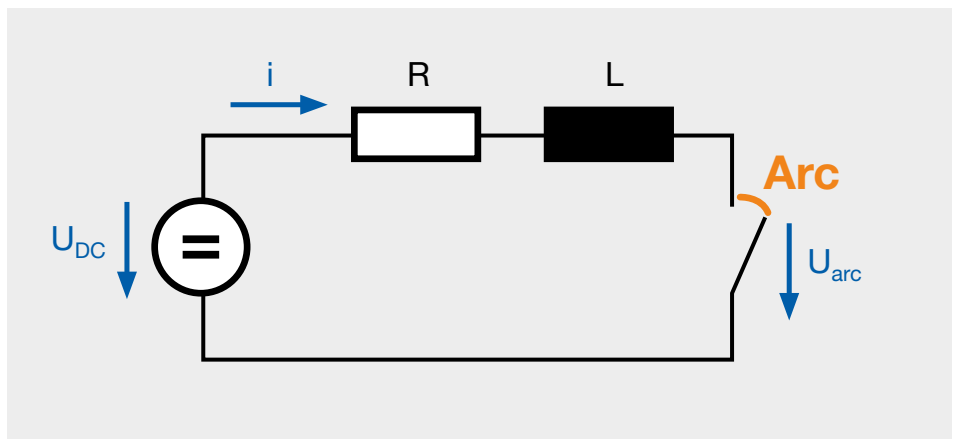
Figure 1: Principle of arc quenching in DC circuits [1]
